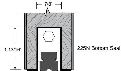
ACOUSTICAL DOOR AUTOMATIC DOOR BOTTOM (supplied with door) Aluminum with neoprene insert 3/4" (19mm) maximum drop
